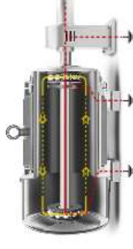
Capacitive EDM Currents and High Frequency Circulating Currents
